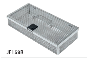
Mini-Size Tray for micro instruments fits into an Aesculap Mini container JK188 or JN188. Length x Width x Height (in.) Outside dimensions 10½ x 5 x 2
